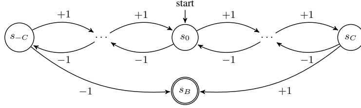
Figure 1. Automaton \mathcal{A}_C .
