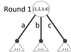
Figure 1: A game tree.
