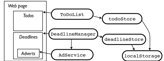
Fig. 1. A mashup for writing scientific papers. The page layout is shown on the left (which also depicts the DOM representation of the page). Rounded boxes are components; arrows indicate object references.
