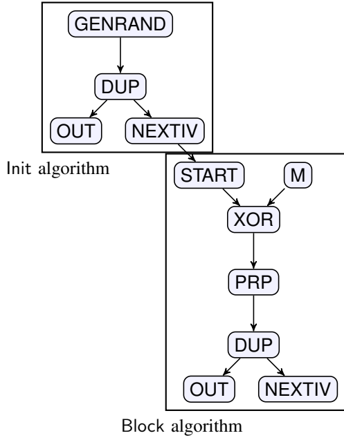
Fig. 2. CBC mode expressed as a graph.
