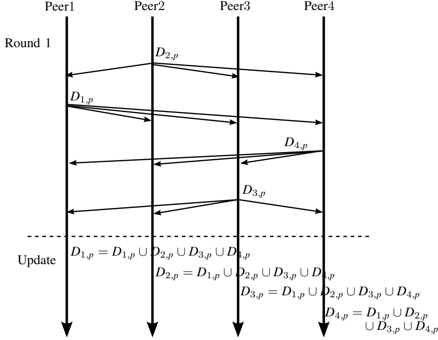
Fig. 3. Fallback Protocol
