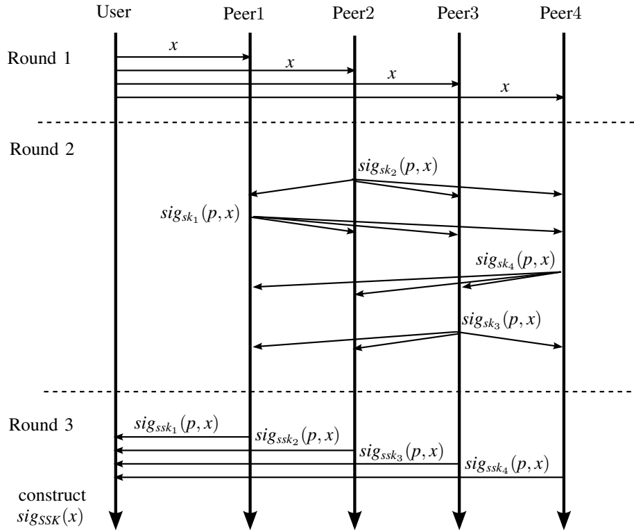
Fig. 1. Posting Protocol
