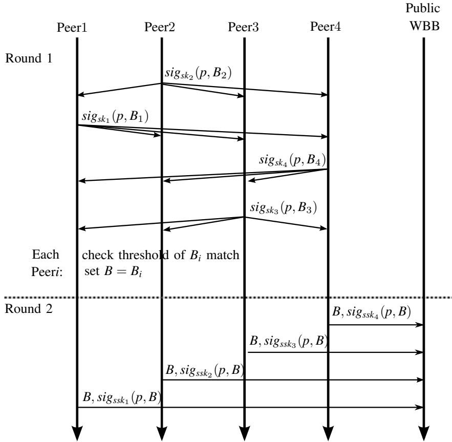
Fig. 2. Optimistic Protocol
