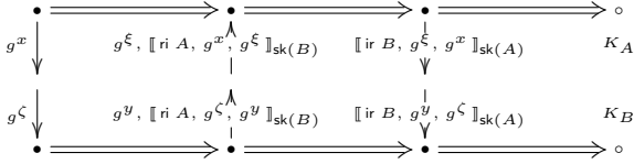
Fig. 3. Variant of the Station-to-Station protocol
