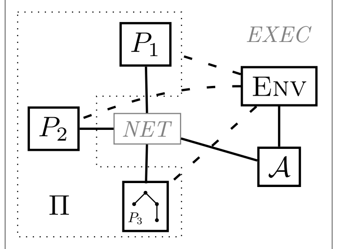
Figure 1: The Communication Model in TUC. The party P_3 exemplifies the machine tree that exists in each party.
