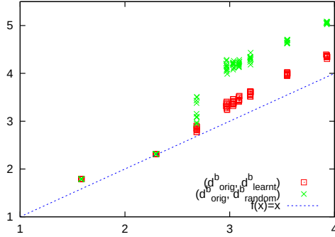
Fig. 6. Relation between the original fractal dimension d_{orig}^b , and the dimension d_{learn}^b after adding learned clauses, or after adding random clauses d_{rand}^b , in random 3CNF formulas. Learnt clauses are computed after 10^3 conflicts.
