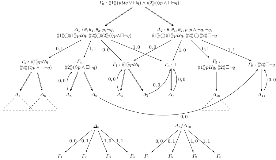
Fig. 2. The pretableau for \theta
