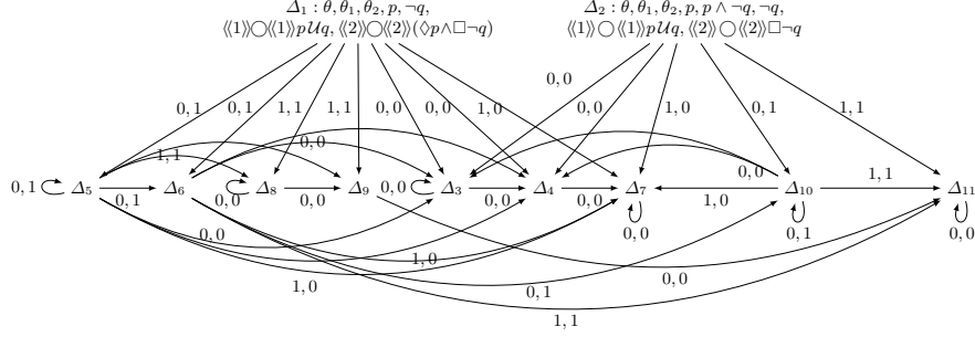
Fig. 3. The initial tableau for \theta
