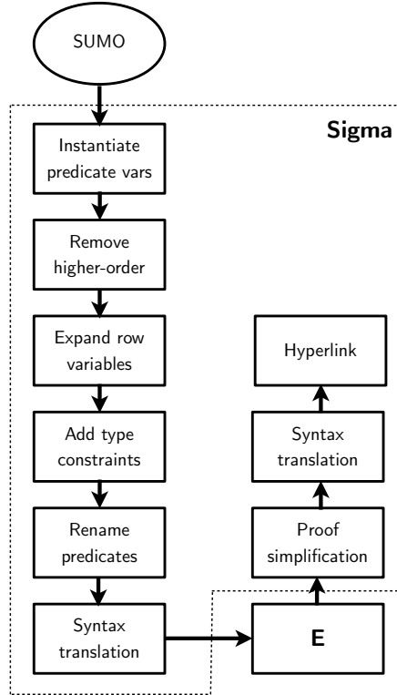
Fig. 2. Language transforms
