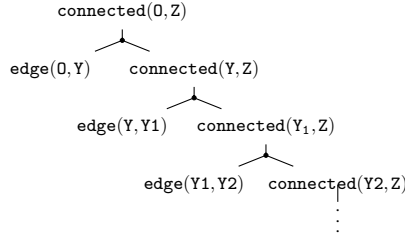
Fig. 4. The infinite coinductive tree for the program GC from from Example 3.1, for the database \text{edge}(0, 1) \leftarrow .
