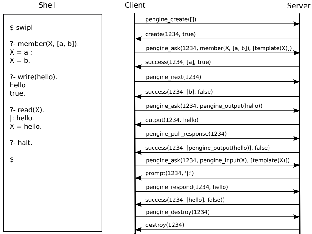
Fig. 2. The PLTP run (on the right) corresponding to a user's interaction with Prolog (on the left). '1234' is the Engine's identifier, which is a UUID in the actual implementation.
