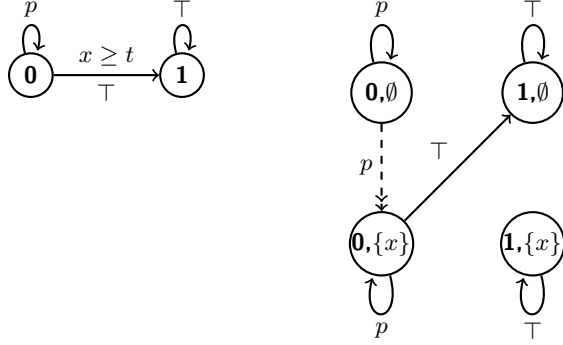
Figure 4. Concrete and symbolic automaton recognizing the language of the PLTL □ formula \Box_t p . The dashed arrow represents a slow transition.
