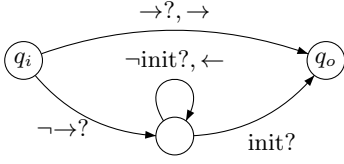
Figure 1. Guide for the searchable class of finite (nested) words
