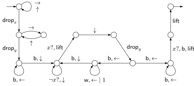
Figure 2. Weighted pebble walking automaton \mathcal{A} computing the size of the largest frame in a picture.
