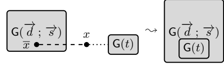
Figure 11. Axiom reduction
