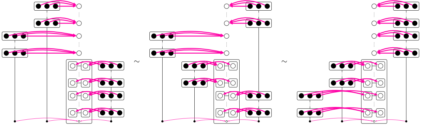
Figure 5. Rewiring three edge-gadgets connected to a single vertex-gadget
