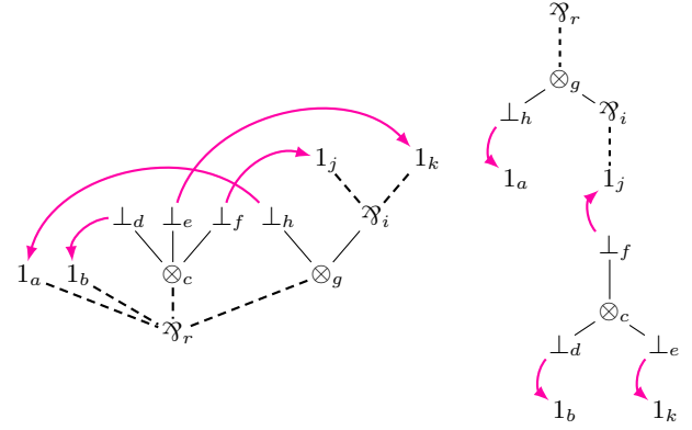
Figure 6. A switching graph of a proof net as a directed tree
