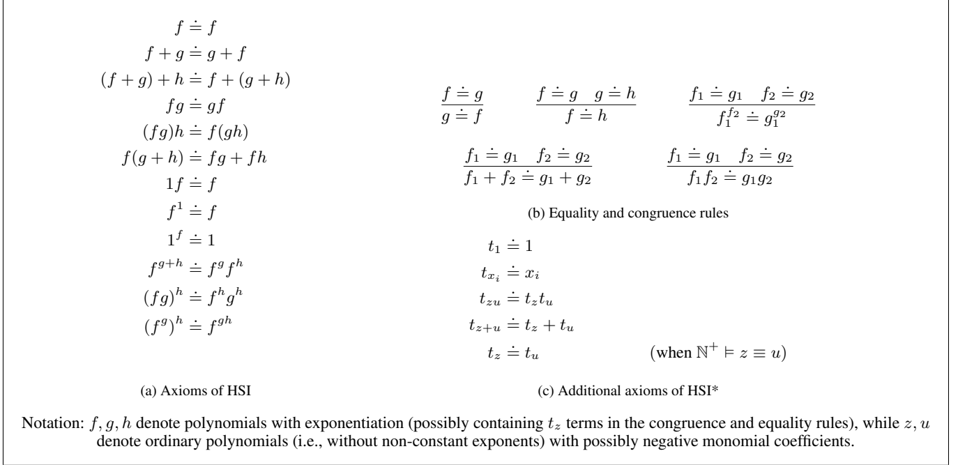
Figure 1: The derivation system of (Extended) High-School Identities
