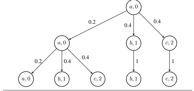
Figure 2. A sample probabilistic tree
