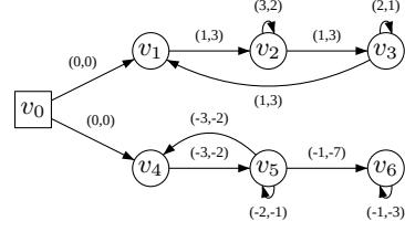
Figure 5. Game graph G .
