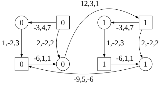
Figure 2. Game graph G according to strategy \sigma .
