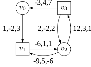
Figure 1. Game graph G . Player 1 owns the round vertices.
