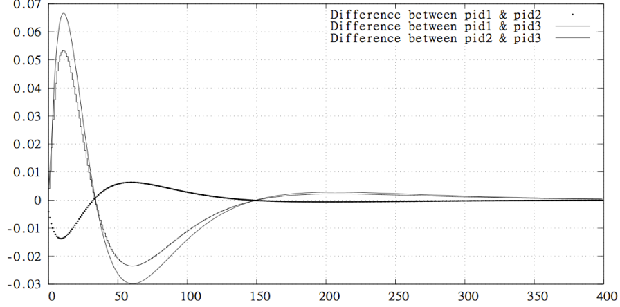
Fig. 2. Difference between the values of the measure m in the three PID.
