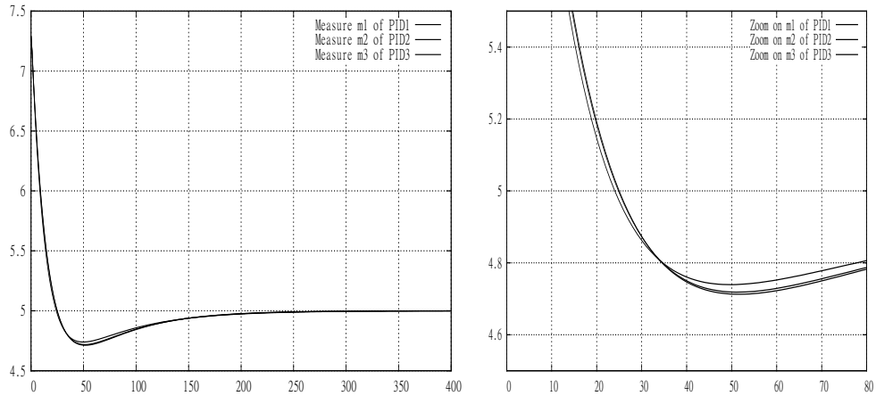
Fig. 1. Value of the measure m in the three PID algorithms.
