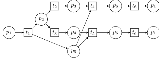
Figure 2: Branching process of PN_1
