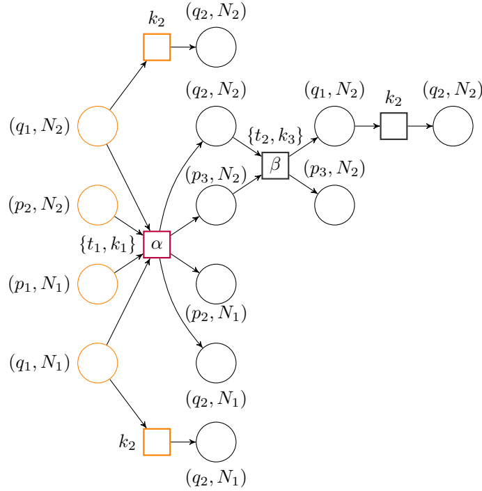
Figure 8: Complete branching process BP_c of NP_2
