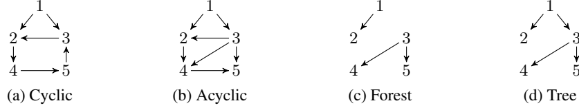
Fig. 1: Directed example graphs with five vertices each
