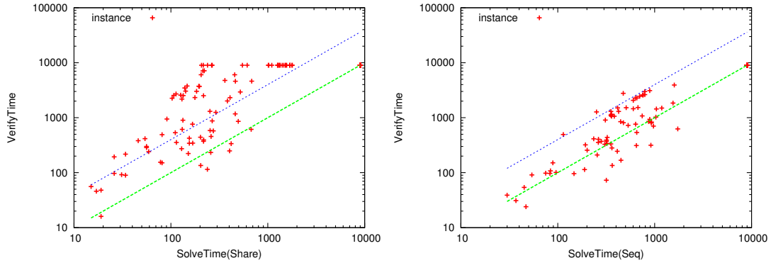
Figure 4: Solving time compared to verification time for the clause sharing portfolio (left) and the sequential solver (right).
