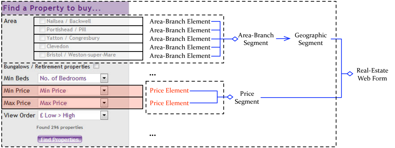
Figure 2: Annotated Example Form (Heritage)
