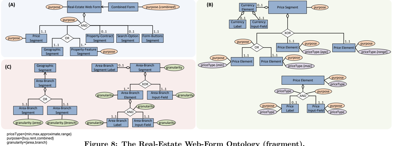
Figure 8: The Real-Estate Web-Form Ontology (fragment).
