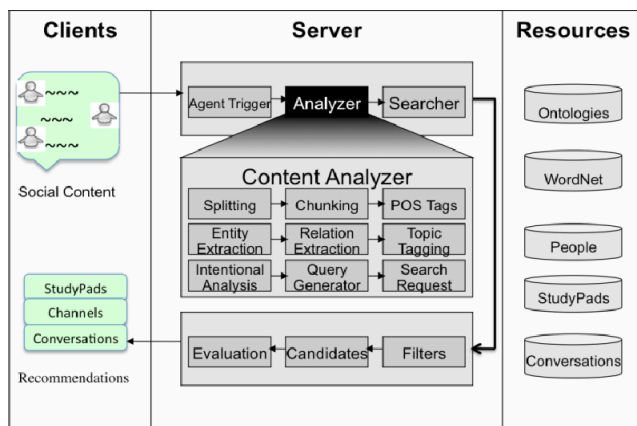
Figure 3. NLP Components.
