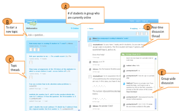
Figure 1. OpenStudy Interface.
