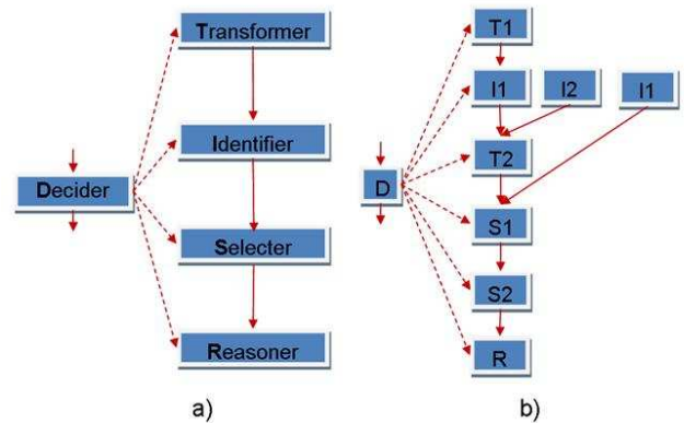
Figure 3. Examples of simple LarKC workflows a) the Urban LarKC Milan Monument Scenario b) a hypothetical branched workflow
