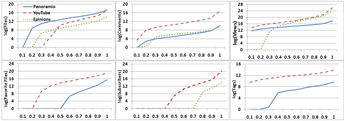
Figure 1: Various factors in the examined WSM. X axis denotes percentage of the users, ranked by the logarithmic attribute value depicted in Y axis.
