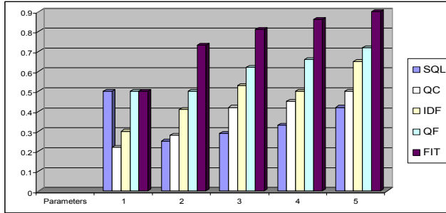
Figure 2: NDCG Comparative results of various ranking methods.
