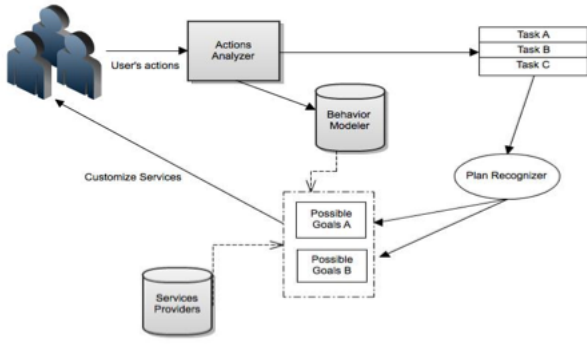
Figure 1: The different elements of the proposed architecture
