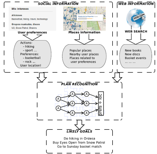
Figure 3: An example of the behavior modeler
