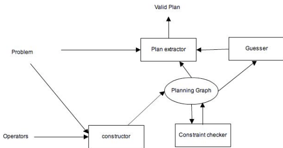
Figure 2: An schema of the plan recognizer module
